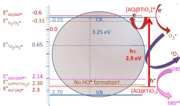
Fig. 6. Proposed mechanical scheme for the synergy effect observed in singlet production by sensitized \text{TiO}_2/\text{AQ@T} (visible light is absorbed by the \text{AQ@TiO}_2 complex).
