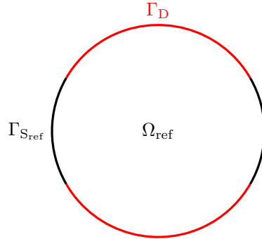
Figure 9.1 – Unit disk \Omega_{\text{ref}} and its boundary \Gamma_{\text{ref}} = \Gamma_{\text{D}} \cup \Gamma_{\text{S}_{\text{ref}}} .
