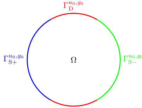
Figure 7.1 – Unit disk \Omega and its boundary \Gamma = \Gamma_N^{u_0, g_0} \cup \Gamma_D^{u_0, g_0} \cup \Gamma_{S-}^{u_0, g_0} \cup \Gamma_{S+}^{u_0, g_0} .
