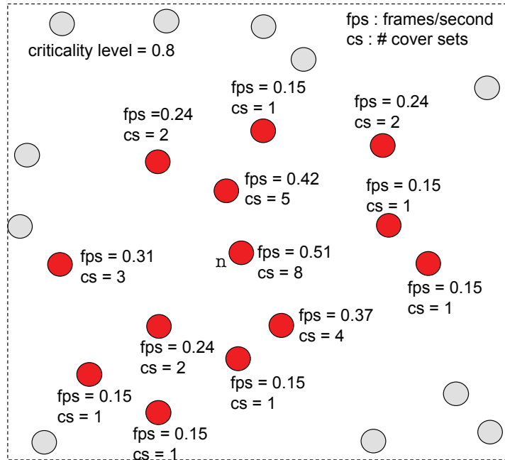
Figure 3.11: Node's frame capture rate under the criticality scheduling with criticality level 0.8.
