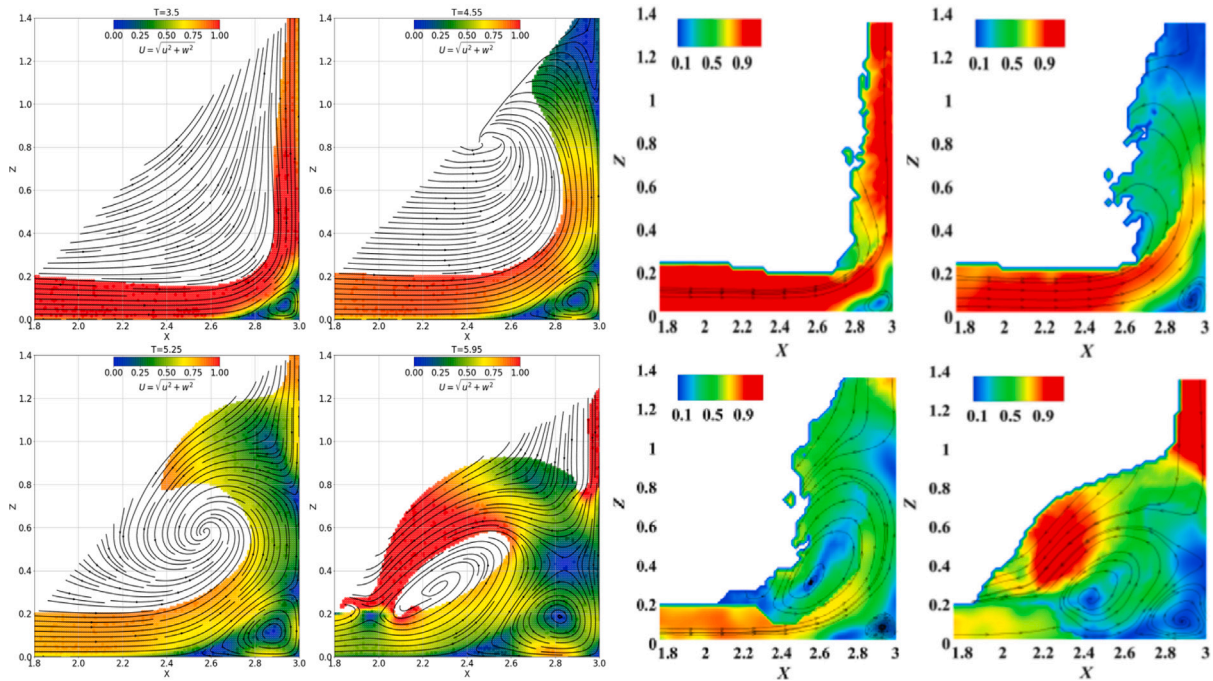
Fig. 25. Velocity magnitude distribution ( U = \sqrt{u^2 + w^2} ) and streamlines calculated by interFoam -3D in the central cross section (left) and measured by Tan et al. (2023) (right) in the central section at the same instants.
