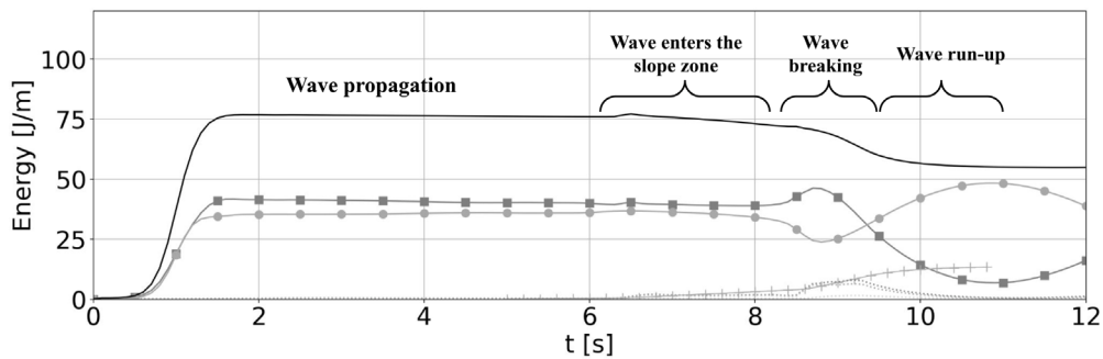
Fig. 15. Time evolution of the wave energy components in the breaking solitary wave case. The simulation is performed with the k - \omega SST buoyancy modified turbulence model of Devolder et al. (2017). The cell size = 5 mm. solid line: E_k + E_p , grey line with \circ : E_k , grey line with \square : E_p , and grey line with '+': integrated dissipated energy.
