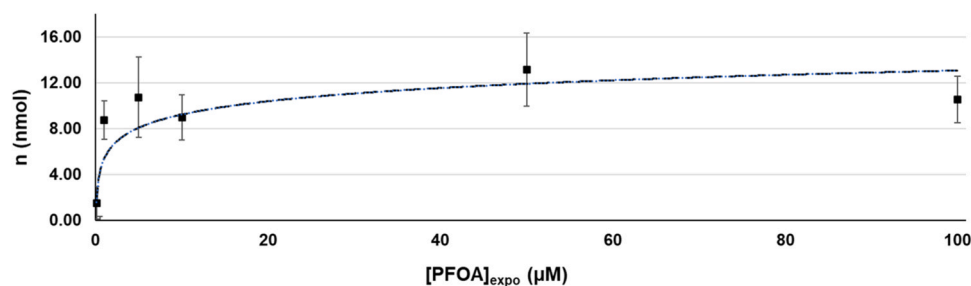
Fig. 7. Quantity of PFOA in the Caco-2 cell monolayer (deduced from Fig. 4 and Eq. 1).
