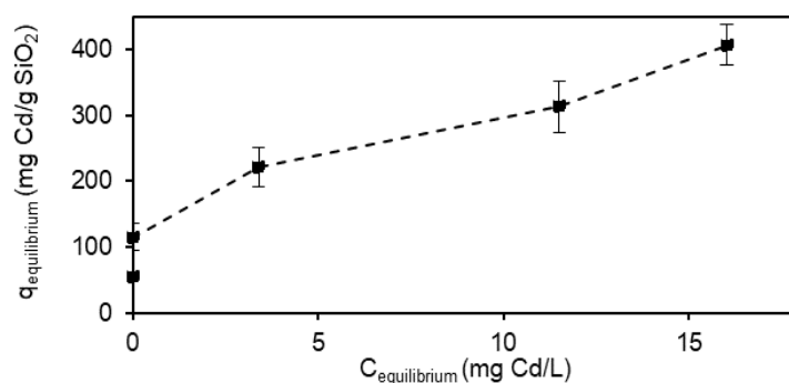
Figure 11. Adsorption capacity ( q ) of Cd by RH2-SiO 2 at different equilibrium concentrations. Equilibrium time was 3 h, concentration of silica 0.2 g/L. Initial concentrations of Cd in MQ water from 0 to 100 ppm. Quantification made by ICP-MS.
