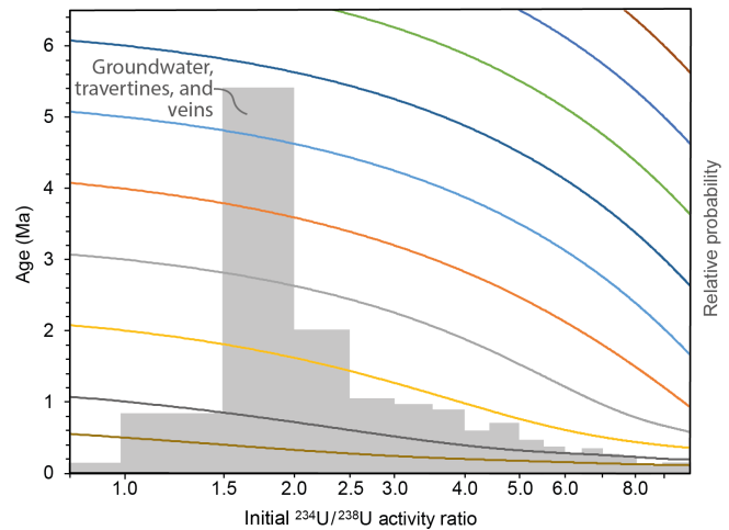
Figure 13. Curves in different colours showing how an individual ^{206}\text{Pb}/^{238}\text{U} age (y axis) will vary with a change in the initial ^{234}\text{U}/^{238}\text{U} activity ratio (x axis). For example, a sample providing a measured ^{206}\text{Pb}/^{238}\text{U} age of 5 Ma will actually have a true age of 3.1 Ma if the initial ^{234}\text{U}/^{238}\text{U} is as high as 6. The grey histogram shows the combined compilations of groundwater, travertine, and vein data from Fig. 12.
