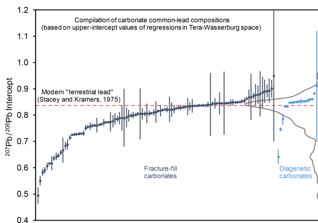
Figure 10. Compilation of upper-intercept ^{207}\text{Pb}/^{206}\text{Pb} compositions from fracture-fill and diagenetic carbonates, of samples dated in the British Geological Survey laboratory ( n = 123 ). The grey curve is a kernel density estimate showing the distribution of mean compositions. The red bar shows the Stacey and Kramers (1975) composition of terrestrial lead in the present day. Samples with very large uncertainties in the ^{207}\text{Pb}/^{206}\text{Pb} composition are those with very low Pb count rates.
