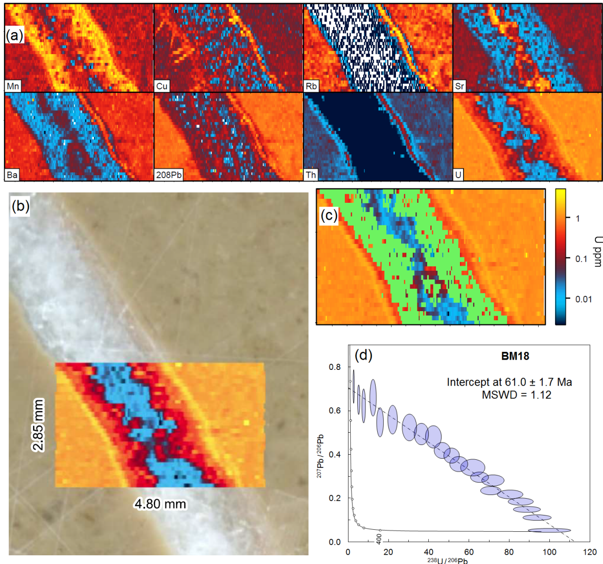
Figure 8. Image-based dating (Monocle plug-in for iolite) of sample BM18. (a) Trace element maps of the analysed region. (b) Photomicrograph of sample surface showing mapped region as U map. (c) U map showing the region of interest selected for the U–Pb date in green. (d) Tera–Wasserburg concordia of U–Pb data after pooling and filtering using the Monocle plug-in (see text for description).
