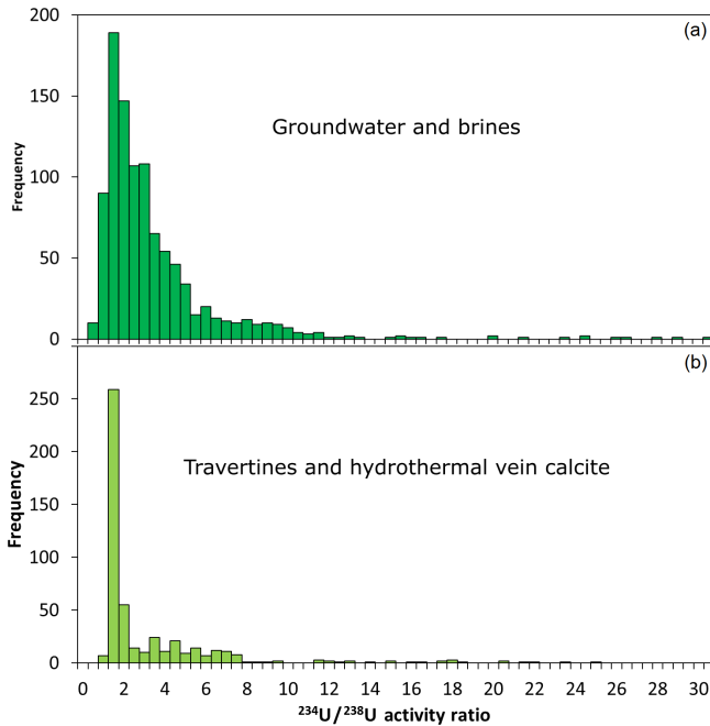
Figure 12. Compilation of uranium ^{234}\text{U}/^{238}\text{U} activity ratios from the literature of (a) groundwater and deep brines – these are present-day ^{234}\text{U}/^{238}\text{U} values (note the compilation is dominated by shallow groundwater rather than brines) – and (b) travertines and calcite precipitated in veins, commonly but not exclusively associated with travertines – these are estimated ^{234}\text{U}/^{238}\text{U}_0 values.
