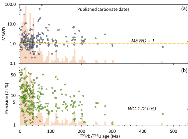
Figure 15. Compilation of published LA-ICP-MS U–Pb dates of carbonate ( n = 318 ). (a) MSWD plotted against ^{206}\text{Pb}/^{238}\text{U} age and (b) precision as 2 s percentage plotted against ^{206}\text{Pb}/^{238}\text{U} age. The histograms in the background show the distribution of dates.
