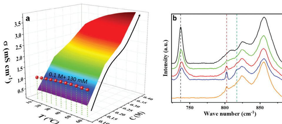
Figure 8. a) Ionic conductivity plots for \text{Mg(TFSI)}_2 in G1:G2 at different concentrations and temperatures. The influence of the \text{Mg}(\text{butyl})_2 additive at 0.1 \text{ M} salt concentration is highlighted with red dots. b) Raman spectra of 0.1 \text{ M Mg(TFSI)}_2 electrolytes with different concentrations of \text{Mg}(\text{butyl})_2 : no additive (black curve), with 50 \text{ mM} (green curve), with 130 \text{ mM} (red curve), and with 190 \text{ mM} (blue curve). The solution without \text{Mg(TFSI)}_2 , containing only 130 \text{ mM Mg}(\text{butyl})_2 in G1:G2 (1:1 vol) is shown for sake of comparison (orange curve).
