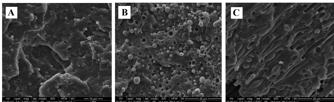
Figure 4. SEM images of r-OPET/rPP blends for different ratios of r-OPET. (A) 10/90. (B) 20/80, (C) 30/70
