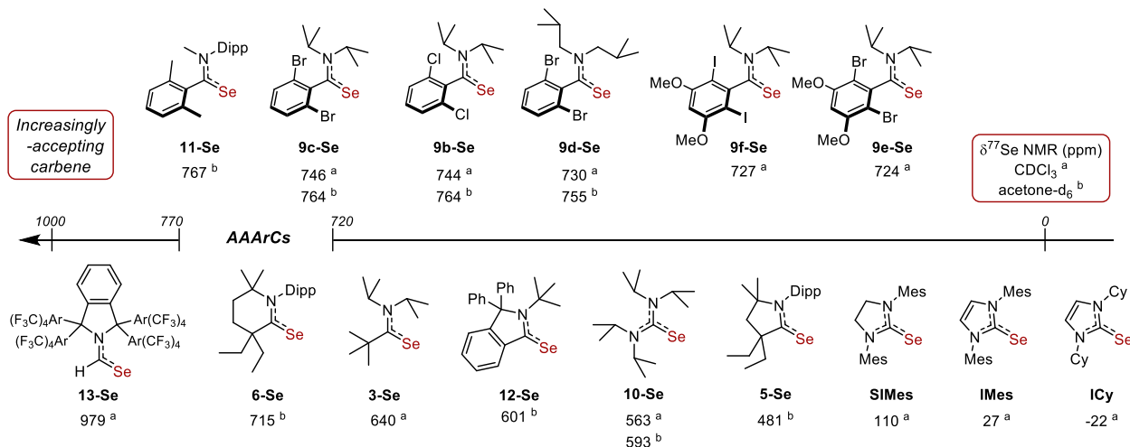
Figure 4. ^{77}\text{Se} Chemical shifts of Se-adducts 9b-f-Se and comparison with representative literature examples of aminocarbenes.
