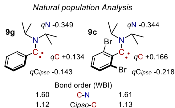
Figure 8. Correlation between NPA charges ( q_C ) on the carbene center, carbene bond angle (in ^\circ ) and the donor-acceptor n_{\sigma}(C) \rightarrow \pi_1^*(Ar) stabilizing interaction in kcal/mol ( \Delta E(2) ). Comparison of the NPA charge distribution and bond order (WBI : Wiberg Bond Index) of the carbene center of 9g and 9c .
