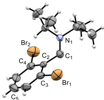
Figure 3. X-ray diffraction crystal structure of 9c (ellipsoids are drawn at 50 % probability). N 1 -C 1 1.286(4) Å, C 1 -C 2 1.469(5) Å, C 3 -Br 1 1.888(4) Å, C 4 -Br 2 1.898(4) Å, αN 1 -C 1 -C 2 117.88°, αN 1 -C 2 -C 5 172.52°, torsion N 1 -C 1 -C 2 -C 3 -94.92°, angles sum around N 1 360.0 °
