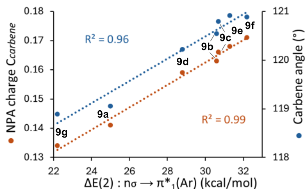
Figure 8. Correlation between NPA charges ( q_C ) on the carbene center, carbene bond angle (in ^\circ ) and the donor-acceptor n_{\sigma}(C) \rightarrow \pi_1^*(Ar) stabilizing interaction in kcal/mol ( \Delta E(2) ). Comparison of the NPA charge distribution and bond order (WBI : Wiberg Bond Index) of the carbene center of 9g and 9c .
