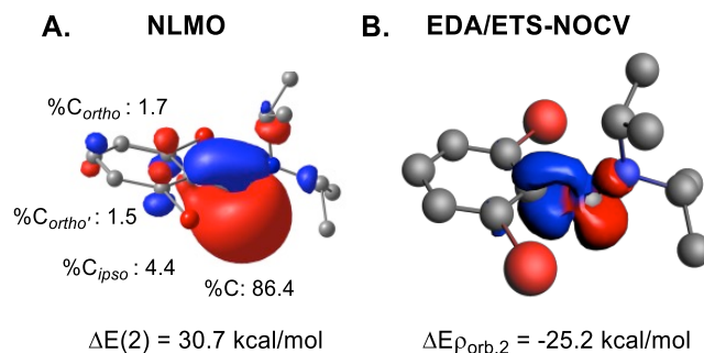
Figure 9. Visualization of the n_{\sigma}(C) \rightarrow \pi_1^*(Ar) delocalization using NBO and EDA/ETS-NOCV analyses. A) Plot of the NLMO (cut-off 0.03) and contributions of mains atoms in %. Stabilizing interaction \Delta E(2) . B) Plot of the contour of deformation density contribution \Delta \rho_{orb,2} of the main pairwise orbital interaction involving the carbene center and associated orbital interaction energy contribution ( \Delta E_{orb,2} ). The charge flow is red \rightarrow blue ( \Delta \rho < 0 in red and \Delta \rho > 0 in blue). The contour value for density is 0.001 a.u.
