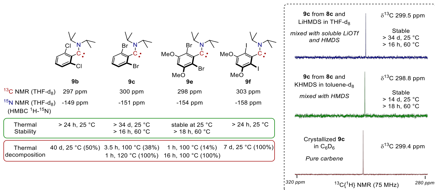
Figure 2. Thermal stability of free acyclic amino(aryl)carbenes and representative 13 C and 15 N NMR signals.
