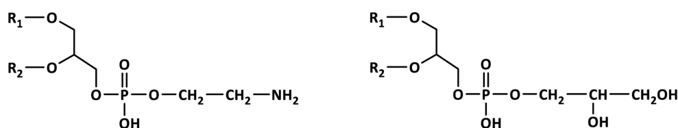
Phosphoethanolamine (PE)
