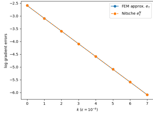
(b) Case 2 with h = 2.5 \times 10^{-2}
