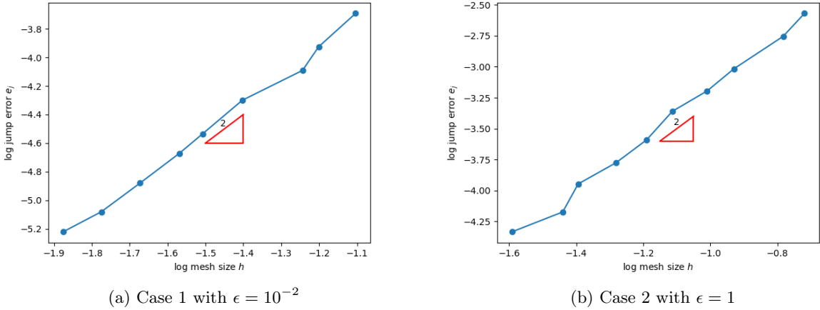
Figure 5: Logarithm plot of the jump error e_j with respect to the mesh size h
