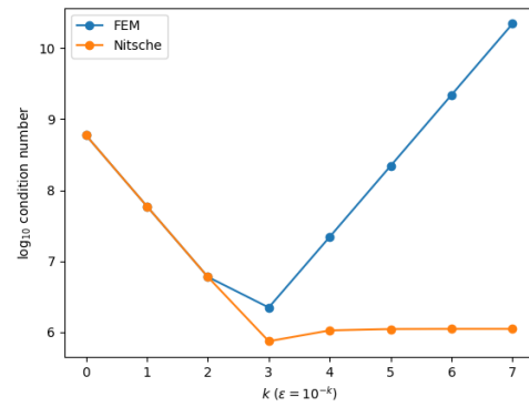
(b) Condition number of case 2 with h = 5 \times 10^{-2}
