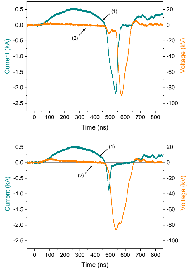
Fig. 6. Waveforms of the current through the diode (1) and voltage at the 49 \Omega load (2) for (a) SOS diode stack (150 kV max) and (b) OTS-150 (150 kV max), with a primary energy E_{C1} of 31.3 J.
