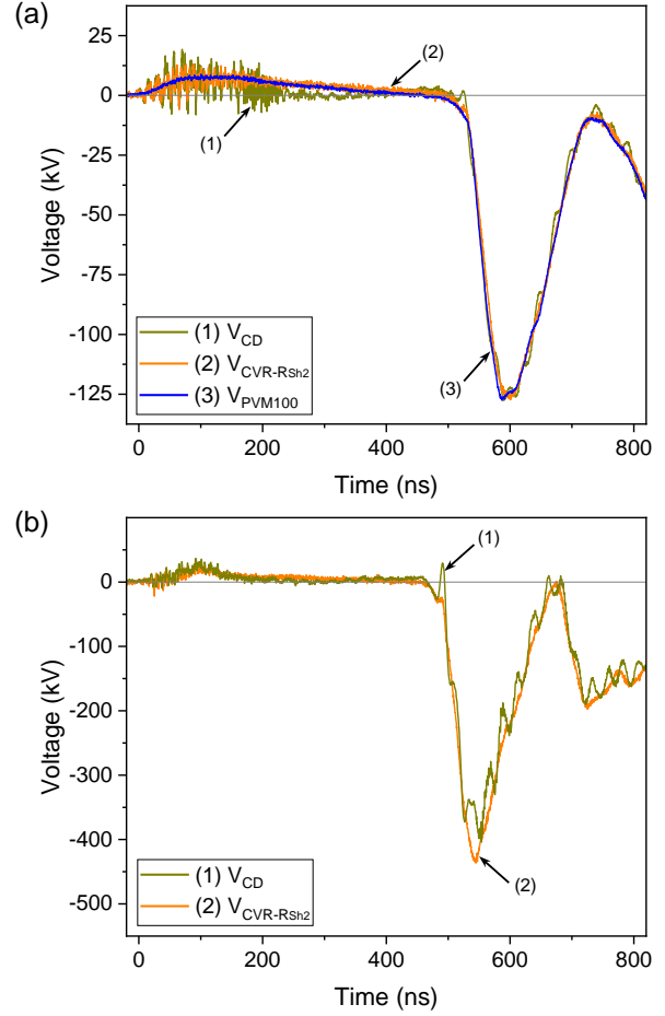
Fig. 8. Load voltage waveforms obtained at 1 k \Omega load, using the capacitive divider CD (1), the current viewing resistor R_{Sh2} (2), and the PVM100 probe (3), for (a) low voltage ( E_{C1} = 4 \text{ J} ) and (b) high voltage ( E_{C1} = 31.3 \text{ J} ).
