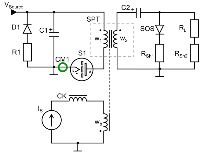
Fig. 1. Circuit diagram of the high-voltage part of the opening switch test bench with an energy stored in C1 of up to 40 J. Description of the components is provided in the text.
