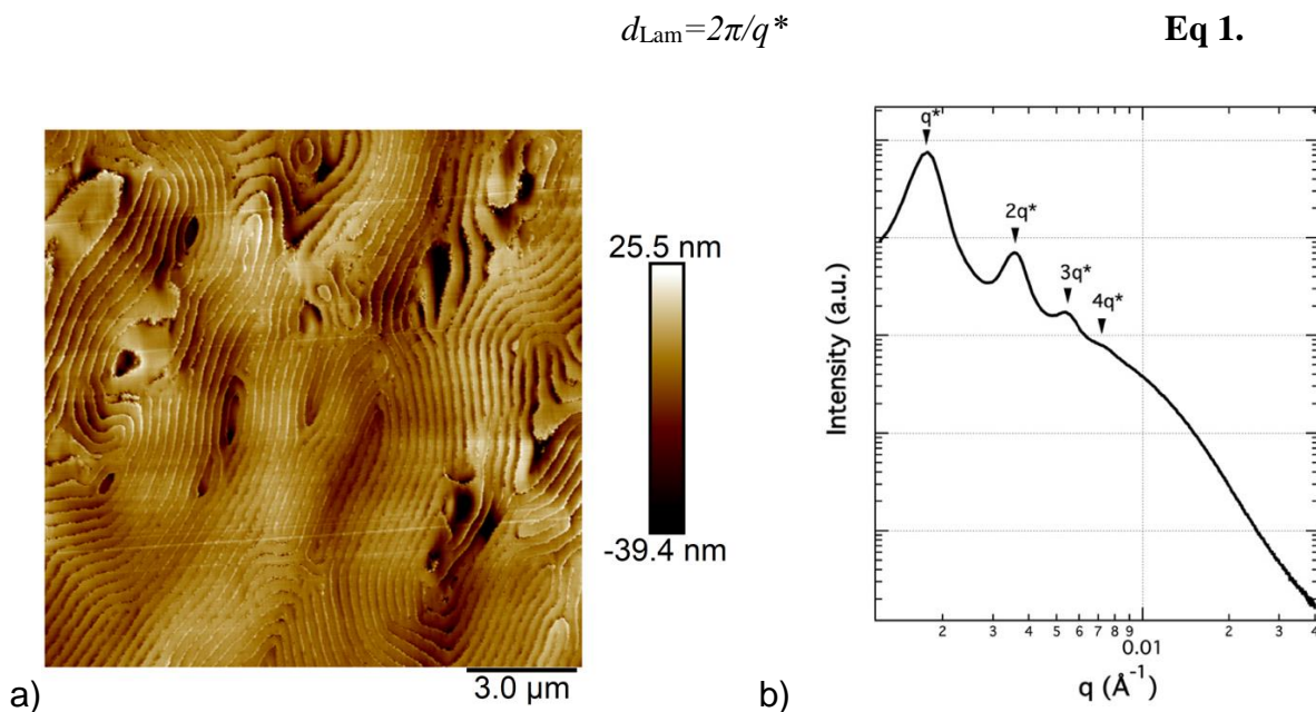
Figure 1. a) AFM height image of s -BCP with the thinner dark phase assigned to P( n BA- co -S) and the thicker bright lamellae to PMMA rich domains. b) SAXS data of s -BCP with peak's assignments.
