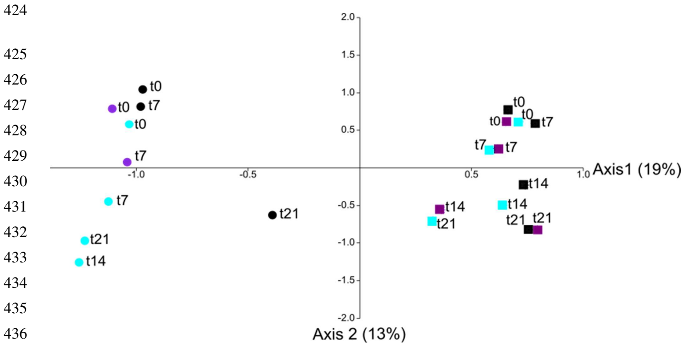
438 Figure 3: Correspondence analysis (CA) comparing microbial communities from pristine (square) and 439 oil-polluted waters (dots) in the three treatments (controls, WAF, WAF+dispersant), at different 440 incubation time. Light blue, Control; Purple, WAF; Black, WAF+dispersant. Numbers indicate the 441 incubation time (days).
