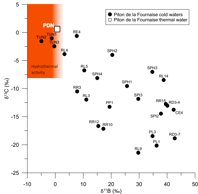
Fig. 3 \delta^{11}\text{B} and \delta^{13}\text{C} isotopic ratios of Piton de la Fournaise waters compared to a thermal water sample from Piton des Neiges. The expected ranges for boron and carbon originating from hydrothermal activity are also represented by the red field 14,34,49,53,55–57 .
