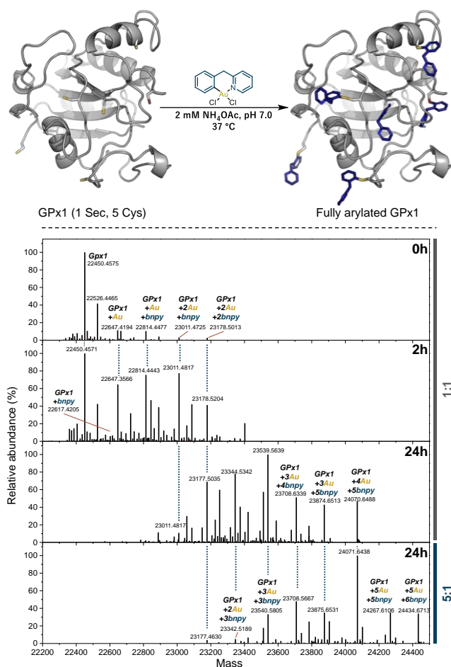
Figure 5. Top: Reaction of GPx1 from Bos taurus erythrocytes with [Au(bnpy)Cl 2 ]. The Sec residue and the 5 Cys residues were assigned as the arylation sites. The bnpy ligand, transferred to the protein upon C-Se and C-S bond formation, are marked in blue. Bottom: The reaction was followed over time under biocompatible conditions (2 mM NH 4 OAc in water, pH 7.0, reaction at 37 °C) and the deconvoluted MS are shown for reaction mixtures at either 1:1 or 5:1 [Au(bnpy)Cl 2 ]:GPx1 ratio. Each peak was assigned based on the number of arylated sites and gold atoms present in the adduct.
