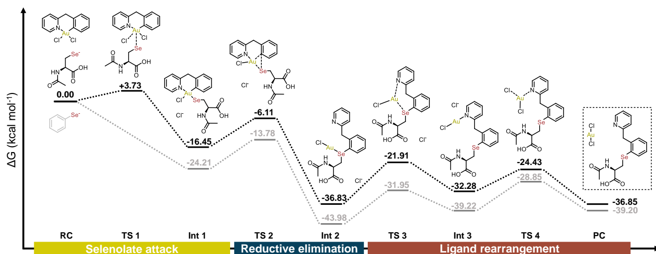
Figure 6. Full Gibbs free energy surface for the Au-promoted C-Se coupling reaction mechanism proposed by DFT at the M06 / 6-311++G(2df,2p) level of theory for non-metal atoms and ECP60MDF / aug-cc-pVDZ-PP for Au. Only the species involving N -acetyl selenocysteinate are fully represented (reaction pathway shown in black), while the species and corresponding energies for phenylselenide are shown in gray. In each system, there is a total of 9 explicit water molecules that are not shown in this simplified diagram for the sake of clarity. For the full structures of each species including explicit water molecules please refer to the supplementary information ( RC = reactant complex; TS = transition states; Int = intermediates; PC = product complex). The reaction coordinate is split in three phases: the attack of the selenolate to the cyclometalated gold(III) compound and incorporation cis to the C-donor; the reductive elimination step, enabling the C-Se coupling; and a ligand rearrangement that allows the release of the gold(I) species.
