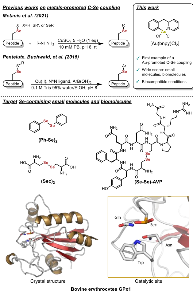
Figure 1. The cyclometalated gold(III) compound [\text{Au}(\text{bnpy})\text{Cl}_2] is used for promoting C-Se coupling across a wide variety of substrates, including under biocompatible conditions. Previous works on metal-promoted C-Se coupling mostly explore copper. [5,10] Here, diphenyldiselenide (Ph-Se) 2 and selenocystine (Sec) 2 were selected as small molecule models. The reaction was also demonstrated with the diselenide analog of the cyclic peptide vasopressin, (Se-Se)-AVP, and the GPx1 selenoprotein from bovine erythrocytes. The GPx1 structure (PDB ID 1GP1) shown highlights the Sec-containing catalytic site (note that in the crystal structure, the Se atom is present in an oxidized state). [23]
