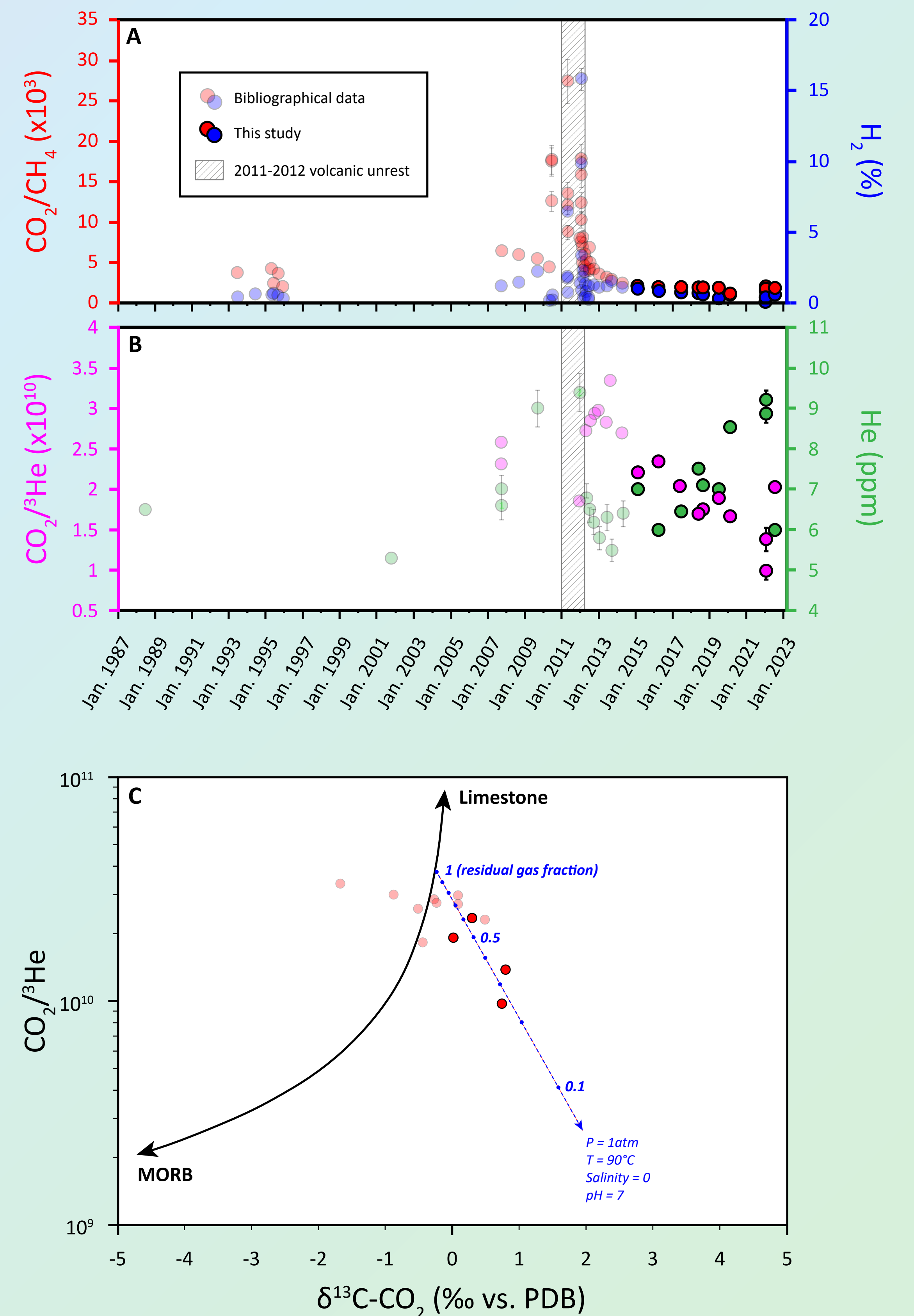
Figure 3 : A) Temporal evolution of \text{CO}_2/\text{CH}_4 ratio, and \text{H}_2 concentration. B) Temporal evolution of \text{CO}_2/{}^3\text{He} ratio, and He concentration. C) \text{CO}_2/{}^3\text{He} vs. \delta^{13}\text{C-CO}_2 . Data from January 2022 are personal data, the other come from the INGV (Italy). Blue line represent the path of selective dissolution of gases in water modeled by an open-system condensation process under equilibrium conditions. (cf. Rizzo et al. 2015; 2019, and references therein).
