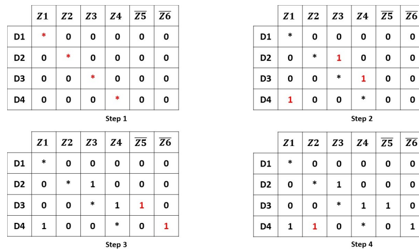
Figure 4. Algorithm steps example with 4 devices, 4 covered (Z1–Z4) and 2 uncovered zones (Z̄5–Z̄6).
