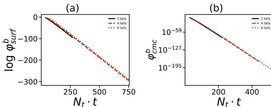
Figure 4. Dependence of (a) the volume fraction (dimensionless) \phi_{surf}^b of free surfactant molecules and (b) the critical micelle concentration \phi_{c.m.c.}^b on the overall number of monomeric units in all tails at different numbers of tails. Data for the same generation number G = 4 are shown.
