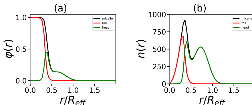
Figure 11. The radial distributions of segments in the hydrophobic core and hydrophilic corona, as well as the total distribution: (a) the volume fraction \varphi(r) and (b) the number distribution n(r) . All cases correspond to the same number of tails t = 2 , tail length N_t = 60 , and generation number G = 4 .
