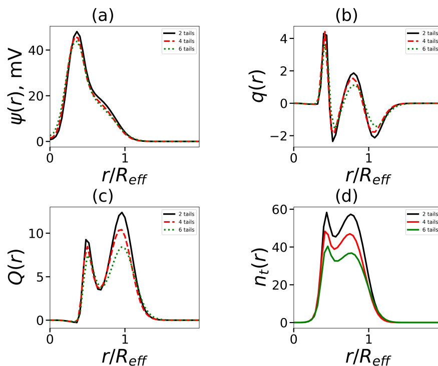
Figure 10. The normalized radial distribution (by effective radius R_{eff} ) (a) the electrostatic potential \psi , (b) the dimensionless charge q(r) , (c) the cumulative charge Q(r) and (d) the terminal charged groups of dendrons in the micelle. All cases correspond to the same overall number of hydrophobic segments in the surfactant N_t \cdot t = 120 ( t = 2, N_t = 60 ; t = 4, N_t = 30 ; t = 6, N_t = 20 ) and generation number G = 4 .
