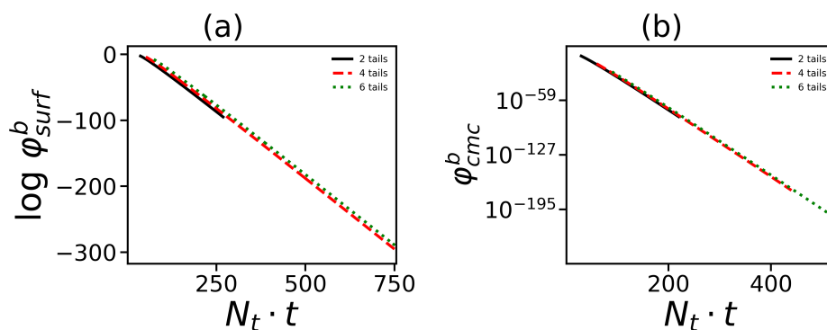
Figure 4. Dependence of (a) the volume fraction (dimensionless) \phi_{surf}^b of free surfactant molecules and (b) the critical micelle concentration \phi_{cmc}^b on the overall number of monomeric units in all tails at different numbers of tails. Data for the same generation number G = 4 are shown.
