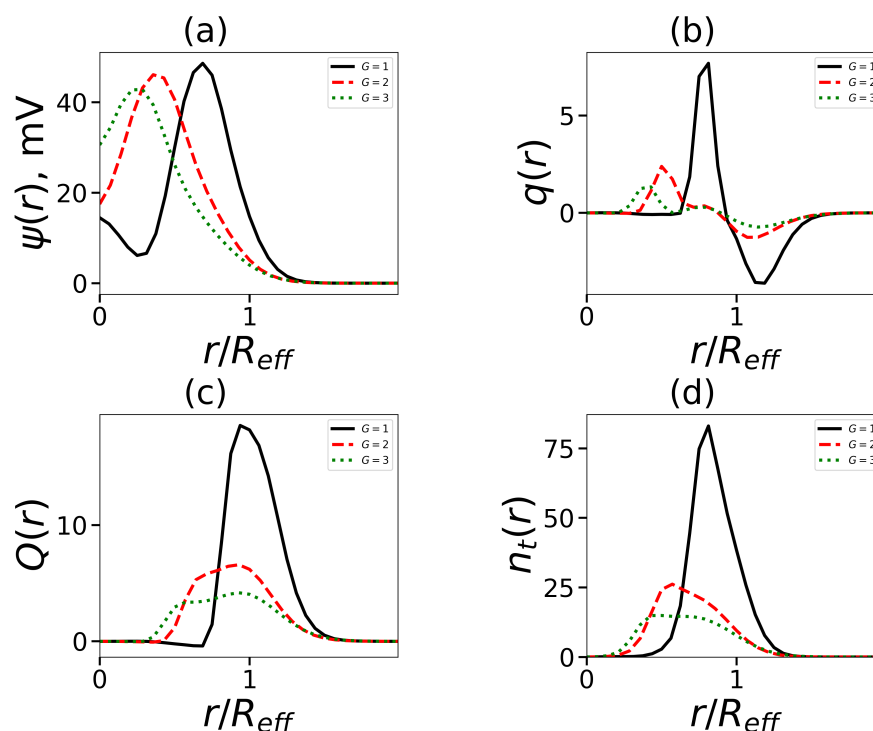
Figure 8. The normalized radial distribution (by effective radius R_{eff} , which is defined below) (a) the electrostatic potential \psi , (b) the dimensionless charge q(r) , (c) the cumulative charge Q(r) , and (d) the terminal charged groups of dendrons in the micelle. All cases correspond to the same number of tails t = 2 , tail length N_t = 15 .
