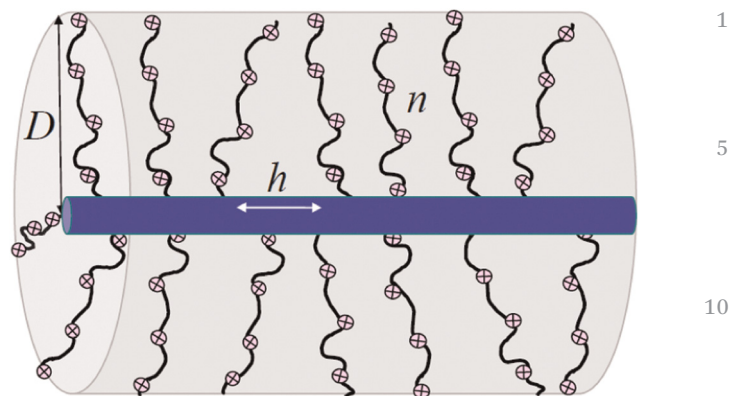
Fig. 1 Schematic of a cylindrical polycationic brush with DP n of tethered polyions and degree of ionization \beta ( i.e. , with number n\beta of charged monomer units per polyion, or equivalently, partial charge e\beta per monomer unit), and linear distance h between neighboring grafts. Mobile ions are not shown.
