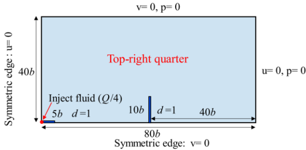
Figure 4: Geometry and boundary conditions after [14], b=0,1m .
