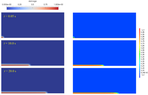
Figure 3: Damage field at different time for the reference model[14] and the proposed model
