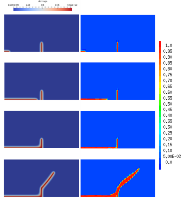
Figure 5: crack pathen left : after [14], right : our model
