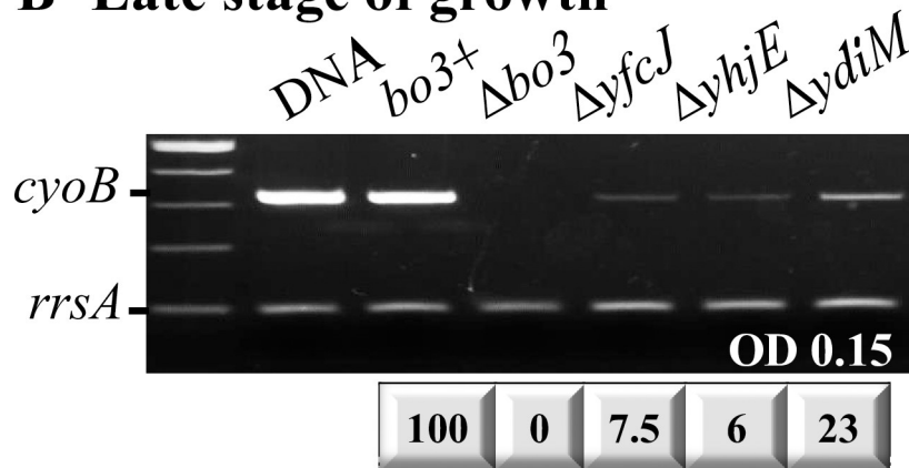
Fig 2. Effects of the absence of YfcJ, YhjE, and YdiM on the transcription of bo 3 -Qox. One step RT-PCR was performed on total RNA extract from bo 3 + strain as well as Δ bo 3 ( cyoB ), Δ yfcJ , Δ yhjE , and Δ ydiM mutants using the cyoB primers to amplify a 322 bp DNA fragment, and the rrsA primers to amplify a 100 bp region of the 16S ribosomal mRNA as a control (Materials and Methods). (A) Early stage of growth. The cells were grown under aerobic conditions at OD 600 of 0.05 (top panel) and 0.1 (bottom panel) where cell division continues. The transcription of cyoB was readily detected and showed no difference at both OD 600 . (B) Late stage of growth. The cells were grown under aerobic conditions at OD 600 of 0.15 (maximum OD 600 reached). The transcripts of cyoB gene were barely detectable when the bo 3 -Qox or the MFS-type transporters YfcJ, YhjE, and YdiM are absent. The numbers below each panel indicate the intensities of the corresponding bands, normalized to that of rrsA then compared to that seen with the
