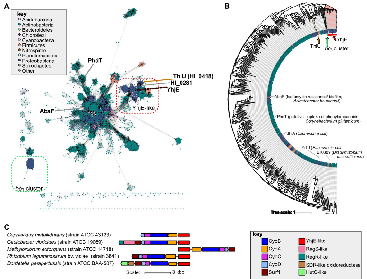
Fig 5. Sequence similarity analysis of YhjE-like transporters and gene neighborhoods containing its homologues. (A) Sequence similarity network using an alignment score of 110. Sequences for the network were collected by searching against UniRef50 (500 hits) with YhjE and mapping to UniRef90 for network construction. Experimentally characterized proteins or proteins with predicted functions (in italics) based on bioinformatic analyses are labeled. The taxonomic classification of each node is colored according to the key shown on top left. (B) iqTREE using edited MAFFT alignment based on UniRef50 sequences, and (C) examples of gene neighborhoods containing a YhjE-like MFS transporter with the key defining them located at the bottom right.
