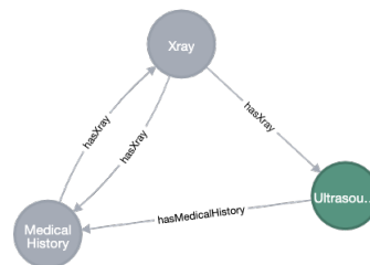
Fig. 6. Generating Summary Graph for query (Q2.3)
