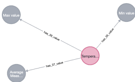
Fig. 7. Generating Summary Graph for query (Q1.3)
