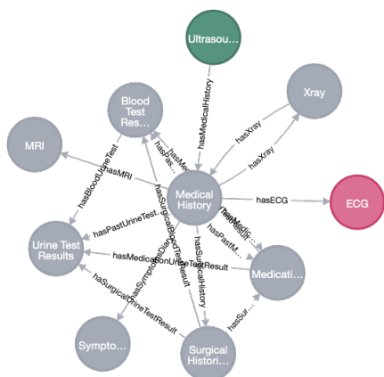
Fig. 5. Generating Summary Graph for query (Q3.3)
