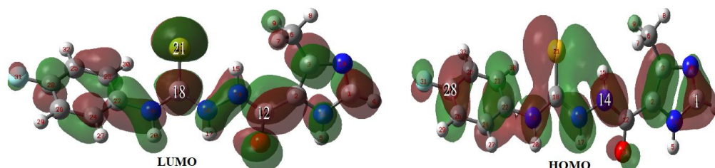
Figure 4: HOMO and LUMO isodensity maps of the ITS 2 compound.
