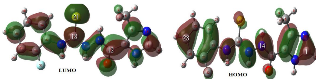
Figure 3: HOMO and LUMO isodensity maps of the ITS 1 compound.
