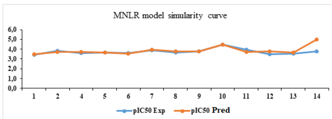
Fig. 5. Evolution curves of the experimental and predicted pIC 50 values of the MNLR model
