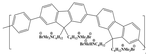
(iv) Cationic Tetrahedralfluorene
