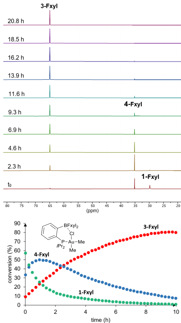
Figure 2. Reaction between the phosphine-borane 1-Fxyl and (AuMe 2 Cl) 2 2 in CDCl 3 at room temperature. Top: Stacked ^{31}\text{P}\{^1\text{H}\} NMR spectra. Bottom: Variation of the relative percentage of P-containing species, as determined by ^1\text{H} NMR spectroscopy.
