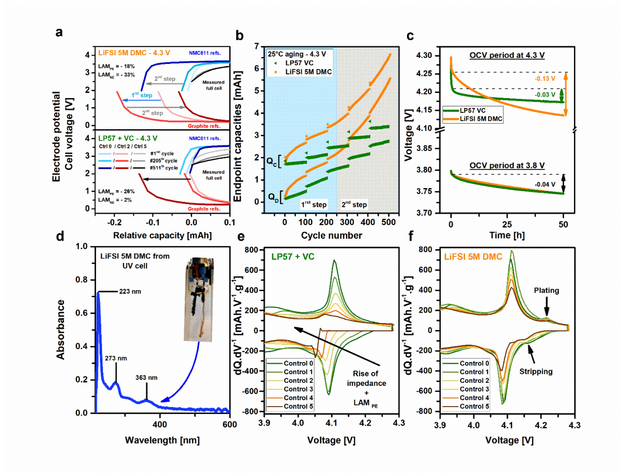
Figure 2: a) Derivative voltage analysis (DVA) of graphite/NMC811 cells cycled using LP57 VC and LiFSI 5M DMC. The control cycles are designated as follows: Control N corresponds to the cycle at C/20 that is measured after subjecting the battery to Nx100 aging cycles at 1C. b) Associated marching capacities. c) Self discharge tests at 3.8 V and 4.3 V. d) UV-visible spectrum of the species released at the positive electrode when using LiFSI 5M DMC electrolyte. Incremental capacity analysis (ICA) performed on C/20 control cycle for LP57 VC e) and HCE-DMC f).
