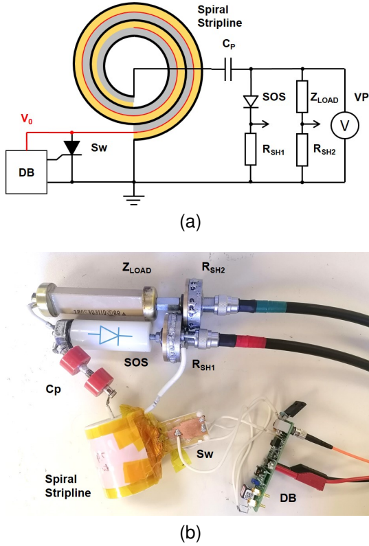
Fig. 4. Circuit diagram of the SG-SOS generator (a) and its configuration based on SOS-60-4 and Z_{LOAD} = 1\text{ k}\Omega (b): Spiral Stripline – spiral pulse forming line, DB – driver board, Sw – solid-state switch, C_p – pumping capacitor, SOS – semiconductor opening switch, Z_{LOAD} – resistive or capacitive load, VP – voltage probe, R_{SH1} and R_{SH2} – resistive shunts.
