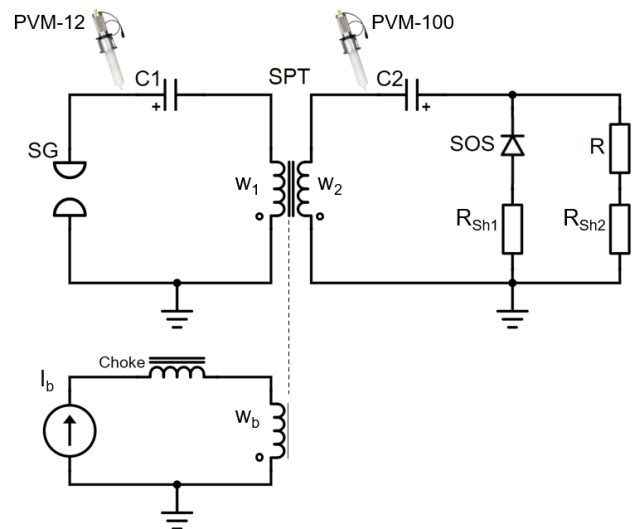
Fig. 1. Circuit diagram of the experimental arrangement.
