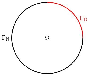
Figure 1: Unit disk \Omega and its boundary \Gamma = \Gamma_D \cup \Gamma_N .
