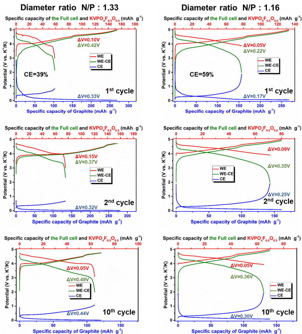
Figure 3. Galvanostatic profiles during the 1 st , the 2 nd and 10 th cycles at C/10 between 3.5-5 V for KVPO 4.9 F 0.5 O 0.5 //graphite 3-electrodes T-cells with N/P diameter ratio of 12.7/9.5 = 1.33 and 11/9.5 = 1.16. The graphite/KVPO capacity ratio was here fixed to 1.16. Note that \Delta V corresponds to the polarization, i.e. the difference between the average potentials.
