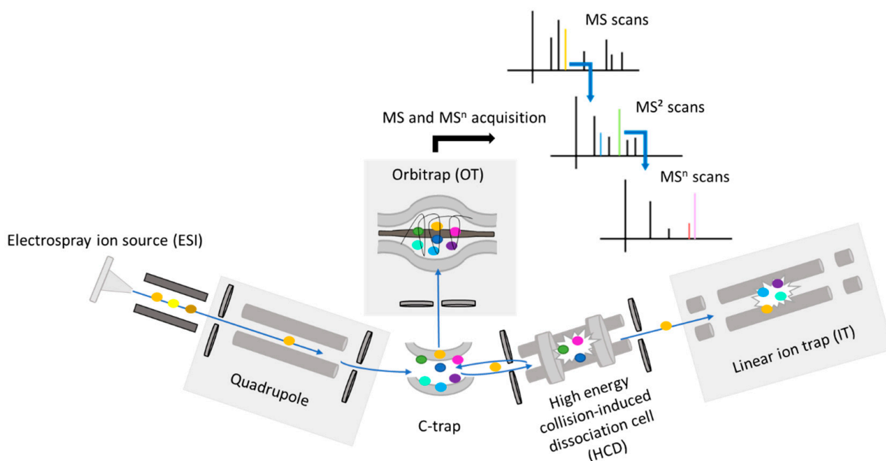
Figure 7. Schematic presentation for Orbitrap Fusion Lumos Tribrid™ mass spectrometer. For data-dependent acquisition, precursor ions were selected in a given mass range by the use of quadrupole as scan filter. Precursors were trapped in the C-trap to be transferred to the Orbitrap for Full MS acquisition. Precursors can also be driven to the high-energy collision dissociation (HCD) cell to be fragmented under drastic voltage conditions or to the linear ion trap (LIT) to perform collision-induced dissociation (CID) fragmentation conditions. Fragment ions are in turn stored to the C-trap and sent to the Orbitrap for their detection. Note that the configuration of such a mass spectrometer permits the achievement of fragmentation levels because of its capability to store fragment ions and simultaneously perform several MS n events.
