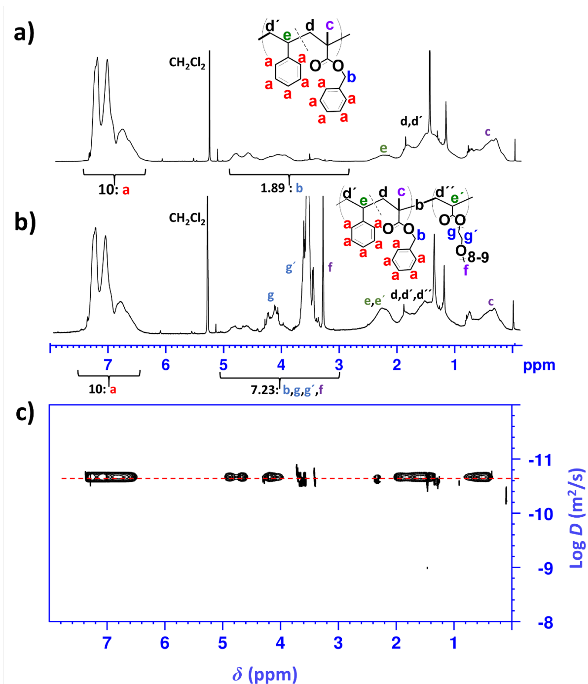
Figure 4. ^1\text{H} NMR spectra of a) s\text{-A}_{0.62} and b) sc\text{-(A}_{0.62}\text{)}_{0.80}\text{B}_{0.20} in \text{CD}_2\text{Cl}_2 ([polymer] = 10\text{ mg}\cdot\text{mL}^{-1} ). Numbers correspond to the integrals of signals. c) DOSY NMR Spectrum: diffusion coefficient ( D ) versus chemical shift ( \delta ) of sc\text{-(A}_{0.62}\text{)}_{0.80}\text{B}_{0.20} .
