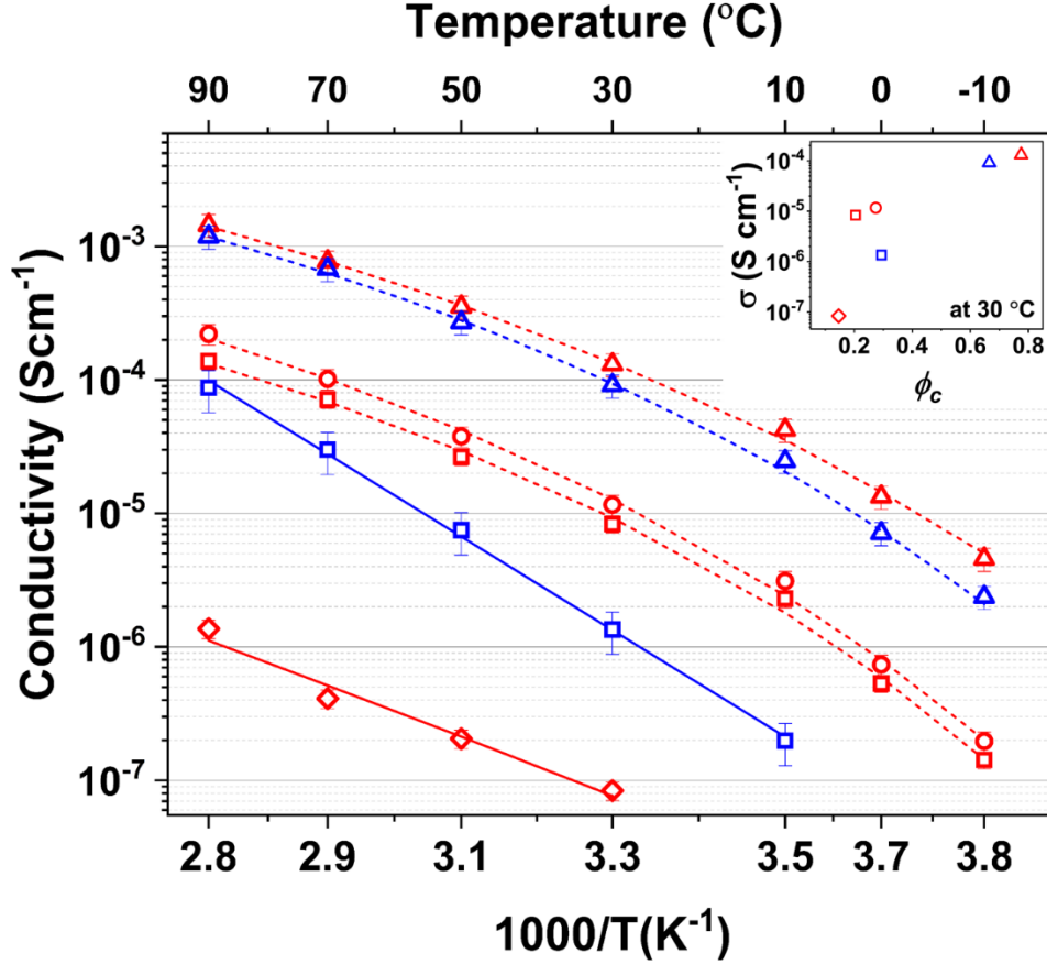
Figure 5. Temperature-dependent ionic conductivity derived from the EIS measurements of BCPEs: ( \Delta ) sc\text{-(A}_{0.62}\text{)}_{0.23}\text{B}_{0.77} , ( \circ ) sc\text{-(A}_{0.62}\text{)}_{0.73}\text{B}_{0.27} , ( \square ) sc\text{-(A}_{0.62}\text{)}_{0.80}\text{B}_{0.20} , ( \diamond ) sc\text{-(A}_{0.43}\text{)}_{0.84}\text{B}_{0.16} , ( \triangle ) lc\text{-(A}_0\text{)}_{0.32}\text{B}_{0.68} , ( \square ) lc\text{-(A}_{0.59}\text{)}_{0.71}\text{B}_{0.29} . Solid lines represent Arrhenius fits and the dashed lines represent VFT fits. Inset graph shows plot of \sigma versus \phi_c of conducting phase for star comb-like (red) and linear comb-like (blue) BCPEs.
