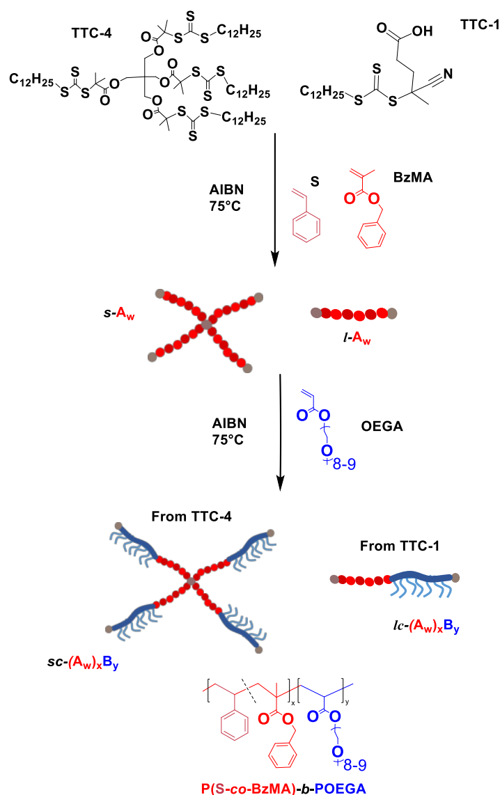
Scheme 1. Schematic illustration of the synthesis route to synthesize lc-(A_w)_xB_y and sc-(A_w)_xB_y block copolymers (BCP) by RAFT polymerization using either TTC-1 monofunctional CTA or TTC-4 tetrafunctional CTA. The A block corresponds to the P(S-co-BzMA) block and B block to POEGA. The subscripts w represents the weight fraction of the BzMA compared to S in the macro-CTA, the subscripts x and y correspond respectively to the weight fractions of P(S-co-BzMA) hard block and POEGA soft block in the AB block copolymer. The prefix lc- and sc- depicts the linear comb-like or star comb-like architecture.
