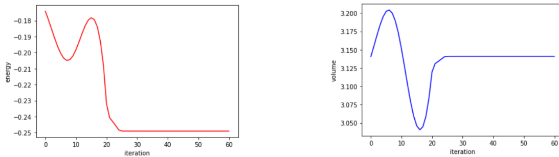
Figure 3: Energy (left) and the volume (right) with respect to the iteration.
