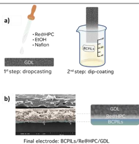
Figure 3. a) Preparation of Re@HPC/GDL and BCPIls/Re@HPC/GDL electrodes. b) cross-section SEM images of 2 wt% in MeOH PS- b -PVBBi TFSI /Re@HPC/GDL electrode dip-coated at 10000 \mu\text{m}.\text{sec}^{-1} .
