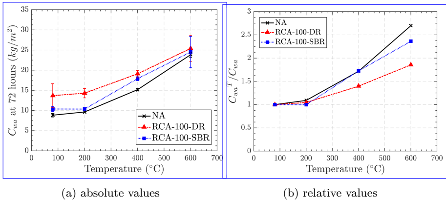
Fig. 4: Evolution of capillary water absorption with temperature
