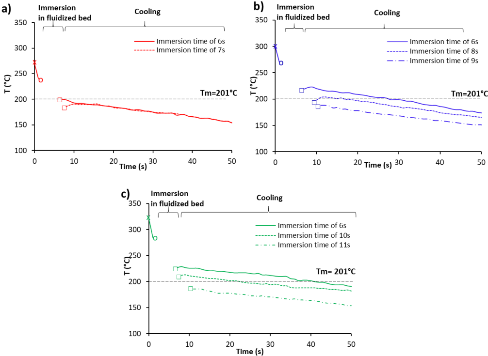
Figure 7 - Evolution of the temperature of coated copper parts preheated to 270°C (a), 300°C (b) and 320°C (c) over the time during the coating process (x : Temperature of the copper cylinder in the oven, o : Temperature of copper cylinder before immersion, □ : Temperature of coated copper cylinder once removed from the fluidized bed)
