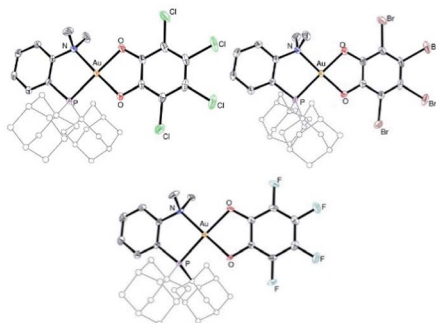
Fig. 2 Molecular structures of the P N Au(III) catecholates 5a–c (for sake of clarity, the substituents at phosphorus are simplified and the hydrogen atoms are omitted).
