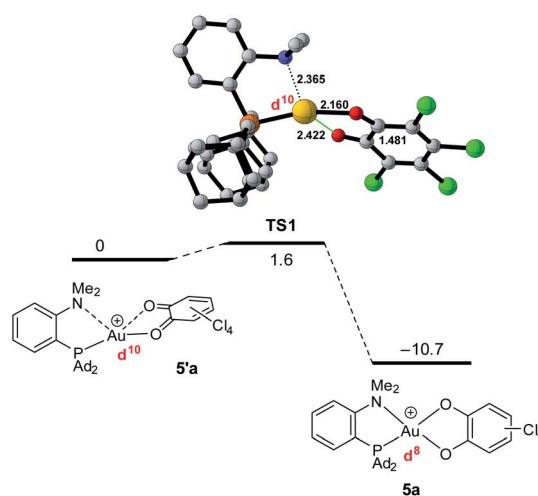
Fig. 6 Conversion of the Au(I) o -quinone valence isomer 5'a into the Au(III) catecholite complex 5a , computed at the PCM(DCM)-B3PW91-D3(BJ)/SDD + f (Au), 6-31G** (C, H, N, O, P, Cl) level of theory.
