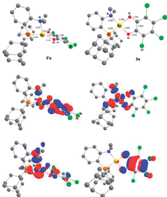
Fig. 5 Optimized geometries of the Au(I) o -benzoquinone ( 5'a , left) and Au(III) catecholite ( 5a , right) valence isomers of the (P N )Au(O Δ O)Cl 4 + complex, computed at the PCM(DCM)-B3PW91-D3(BJ)/SDD + f (Au), 6-31G** (C, H, N, O, P, Cl) level of theory. Distances in Å. Plot of the frontier orbitals with cutoff: 0.05. Hydrogen atoms have been omitted for clarity.
