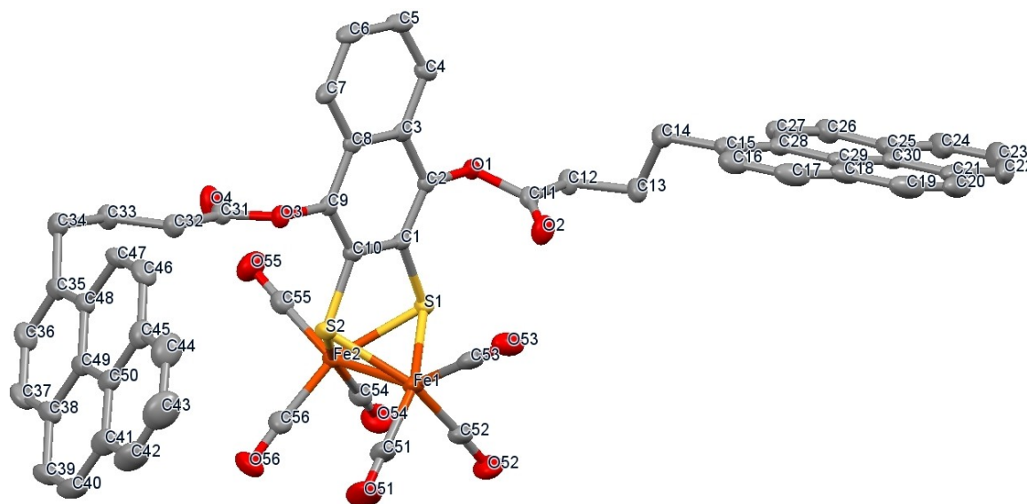
Figure 1. X-ray crystal structure of complex 2 . Color coding: Fe orange; S yellow; C grey; and O red. Hydrogen atoms are omitted for clarity. Thermal ellipsoids set at 50 % probability level. Selected bond distance (Å) and angles (°): Fe1–Fe2, 2.4802(5); Fe1–S1, 2.2598(8); Fe1–S2, 2.2776(8); Fe1–C51, 1.791(3); Fe1–C52, 1.789(3); Fe1–C53, 1.805(3); Fe2–S1, 2.2678(7); Fe2–S2, 2.2743(7); Fe2–C54, 1.793(3); Fe2–C55, 1.806(3); Fe1–C56, 1.796(3); S1–Fe1–S2, 81.24(3); S1–Fe2–S2, 81.13(3). CCDC 2183292 contains supplementary crystallographic data. The asymmetric unit also contains two co-crystallized solvent molecules ( \text{CH}_2\text{Cl}_2 ) which were removed from the figure for better clarity.
