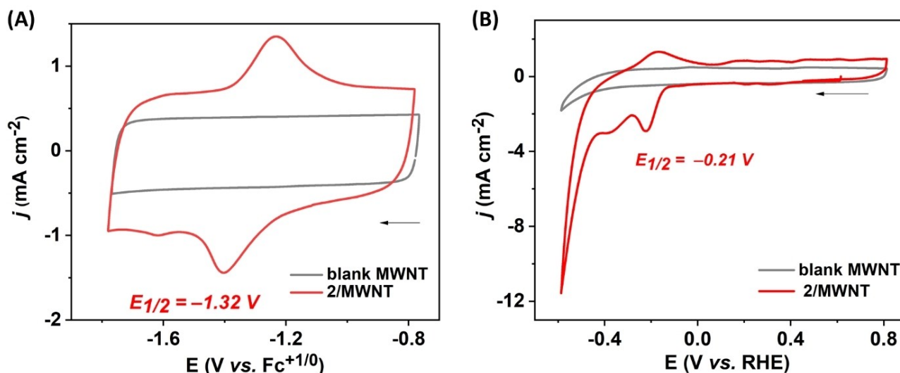
Figure 4. CV traces of the immobilized catalyst (2) in organic and aqueous media. (A) CV traces of complex 2/MWNT (red trace) and the blank MWNT electrode (grey trace), recorded in acetonitrile with 0.1 M TBAPF 6 ; and (B) CV traces of 2/MWNT (red trace) and the blank MWNT electrode (grey trace) recorded in 0.2 M sodium phosphate buffer of pH 7. All CV traces collected at room temperature, \nu = 100 \text{ mV s}^{-1} .
