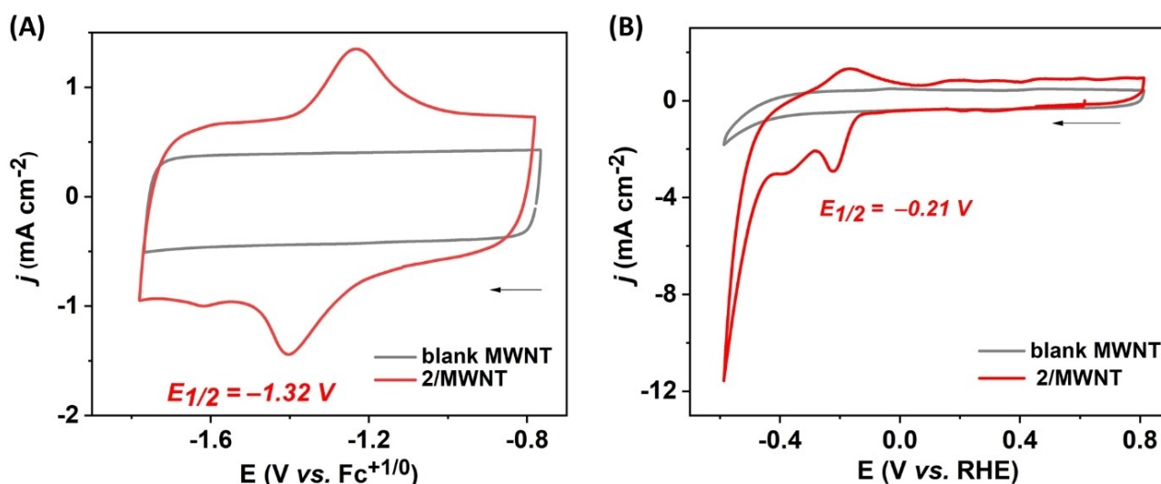
Figure 4. CV traces of the immobilized catalyst (2) in organic and aqueous media. (A) CV traces of complex 2/MWNT (red trace) and the blank MWNT electrode (grey trace), recorded in acetonitrile with 0.1 M TBAPF 6 ; and (B) CV traces of 2/MWNT (red trace) and the blank MWNT electrode (grey trace) recorded in 0.2 M sodium phosphate buffer of pH 7. All CV traces collected at room temperature, \nu = 100 \text{ mV s}^{-1} .
