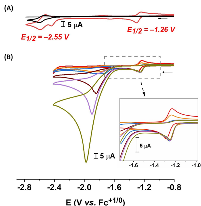
Figure 3. CV traces of 2 (1 mM) under homogeneous condition. (A) Comparison between blank (grey trace), 2 (red trace) and 1-pyrenebutyric acid (black trace); (B) 2 in the presence of different concentrations of trifluoroacetic acid (red = 0 mM, orange = 1 mM, violet = 2 mM, brown = 5 mM, purple = 10 mM, dark yellow = 20 mM). Inset showcases the non-turnover signals as well as onset potentials at different acidic conditions. All CV traces were recorded in DMF, with 0.1 M TBAPF 6 , at room temperature, v = 100 \text{ mVs}^{-1} .
