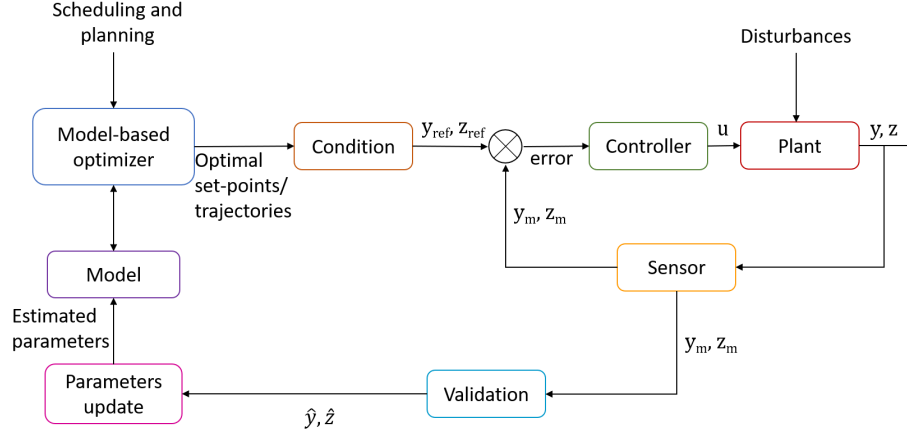
Figure 4: Typical architecture of real-time optimization (based on (Shokri et al., 2009))
