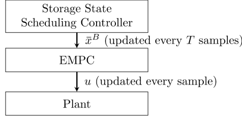
Figure 8: Hierarchical control structure for a system with storage (Clarke et al., 2018)
