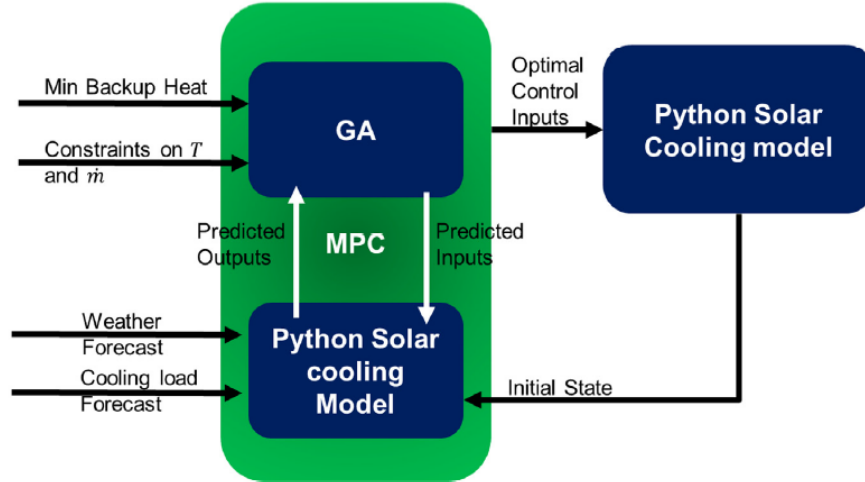
Figure 5: Layout of the EMPC (Pintaldi et al., 2019)
