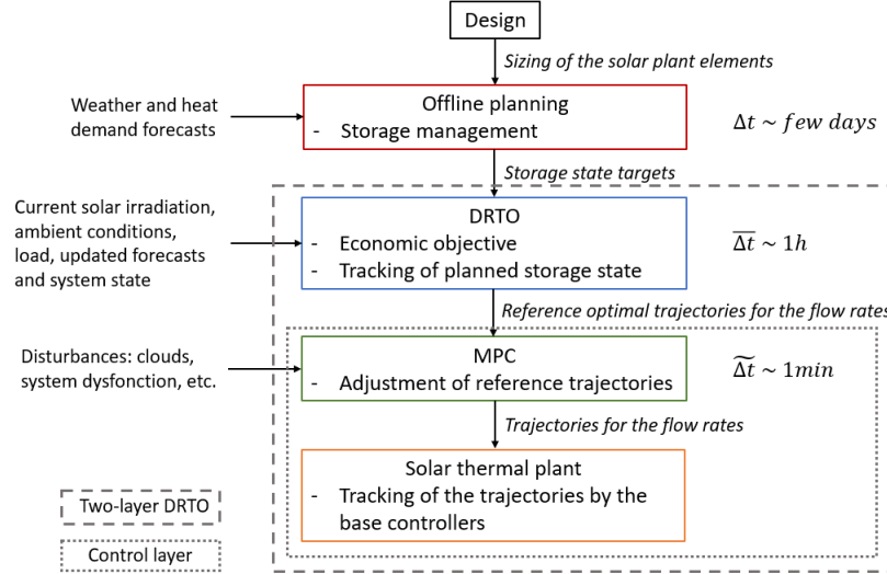
Figure 11: Complete optimization strategy for a solar thermal plant
