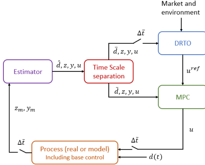
Figure 6: Time-scale decomposition of the disturbances between the DRTO and the control layers (based on (Kadam et al., 2002))
