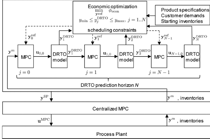
Figure 7: The architecture of a closed-loop two-layer DRTO (Remigio & Swartz, 2020)
