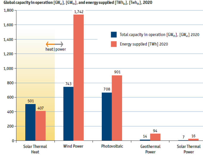
Figure 1: Global capacity and energy supplied for solar thermal and other renewable energy technologies (Weiss & Spörk-Dür, 2021)
