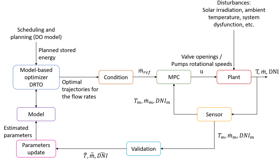
Figure 12: Control diagram for the optimization of a solar thermal plant
