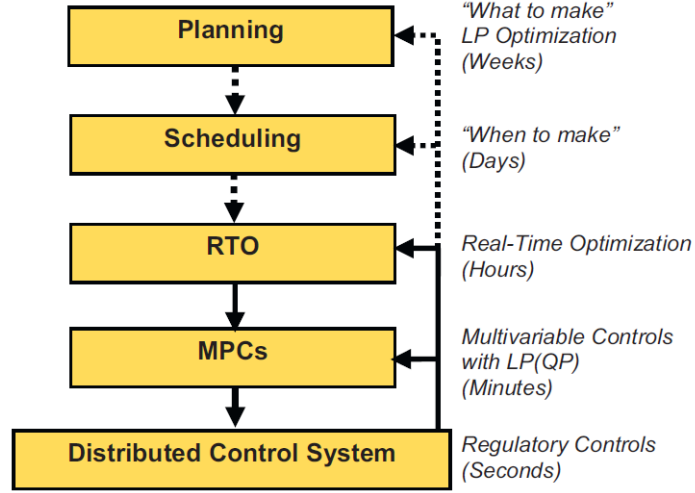
Figure 3: General hierarchy for control and decision making in a plant (Darby et al., 2011)
