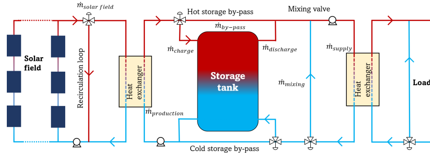
Figure 2: General structure of a solar thermal plant
