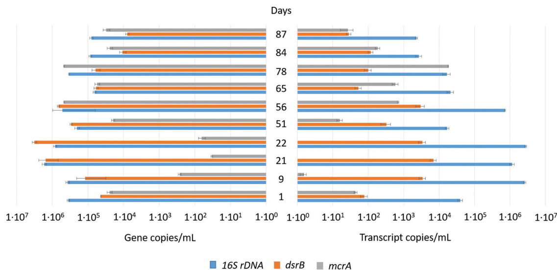
Fig. 6 Quantitative evolution of the microbial community during the incubation at 47 °C, at 85 bar (CH 4 , 1% CO 2 ) before and after hydrogen injection (95 bar with 10% H 2 ). The quantification is estimated by qPCR of 16S rDNA gene copies for each mL of sampled water through the experiment.
